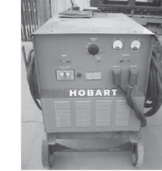
Hobart Mdl 6FR28-400CL GPU, Input: 240/480, Output: 28V, 400 Amps Continuous, 750-1500 Amps Startup
