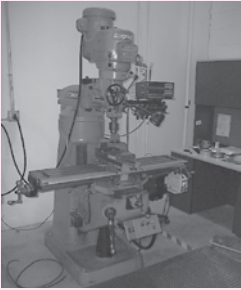
Bridgeport Series I Vertical Milling Machine, 2-HP, 9" x 48", 3-Slot Power Feed Table, 60-4,200 RPM Spindle Speed, Sony Digital X, Y Readout
