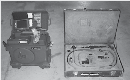
Olympus Iplix SA Series IV7635A Industrial Videoscope System
