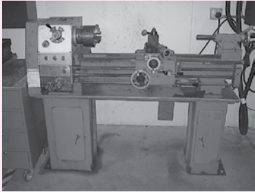
Enco Mdl 110-2072 Gap Bed Lathe, 12" Swing Over Bed, 16" Swing in Gap, 48" Bed, 38" Between Centers, 70-1,220 RPM Spindle Speed
