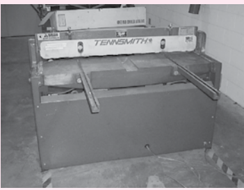
Tennsmith H52 Power Sheet Metal Sheer, 52", 16-Gauge Capacity
