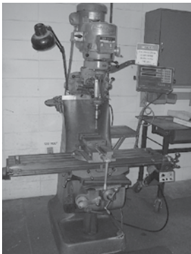
Bridgeport Series I Vertical Milling Machine, 2HP Motor, 9"x 48" 3-Slot Table, Rapid Reverse Attachment, Acu-Rite Master MP Digital X, Y Readout, Vaughan's Sheet Metal Stake Table w/Dies
