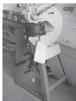
Rotex Mdl 18-A 53' Turret Sheet Metal Hole Punch (2) Beverly No. B-3 Shears
