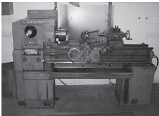
Cincinnati Milacron 13" Hydra Shift Engine Lathe, Swing Over Bed 13-1/4", Swing Over Cross Slide 8-7/8", Distance Between Centers 24" - 60", Spindle Speed 35 - 3000 RPM, 1-3/4" Spindle Hole, w/Taper Attachment
