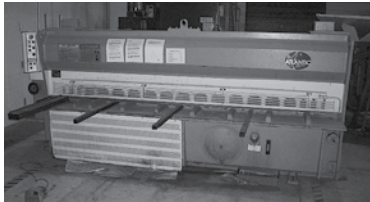
Atlantic Mdl HHDS 10' Power Sheet Metal Shear w/Power Back Gauge & Hyd Hold Downs
