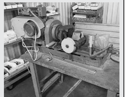
AeroQuip Hose Fitting Machine, 1.5-HP Motor, -3 thru -32 Hoses
