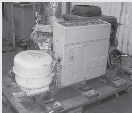
Hawker APU Engine GTCP30-92 Turbine Powered Generator Set w/Solar T41M-9A Engine, 30 KVA Misc Turbine Engine Inventory
