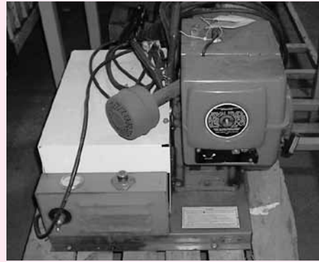
Kohler GSE Jump Start Unit w/Kohler Magnum 10 Gas Engine & Generator Rachem HT-900B Nitrogen Heater
