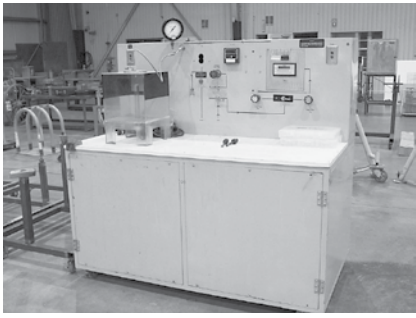
CJ610/CF700 Fuel Nozzle Test Stand w/ Heater/Chiller
