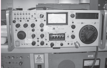
IFR Nav-750B VOR/LOC/Comm & G/S Test Set
