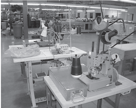
Union Special Mdl 812000 Industrial Sewing Machine Dorina 730 Sewing Machine Juki MO-6700 Industrial Serger NC Carpet Binder Mdl 812003 (3) SU LEE Machine Round Knife Carpet Cutter Mdl RC-280 Eastman 355 Round Knife Carpet Cutter Wolf Round Knife Cutter Bosch Mdl 1575A Foam Saw United-Carr Mdl M235 Foot Operated Grommet Machine Twice As Sharp Pedestal Scissor Sharpener 16' Upholstery Shop Layout Table Several Upholstery Layout Sewing Tables Partial Rolls of Kevlar Cloth, Aluminum Fiberglass & Dry Graphite Mat Misc Rolls of Interior Fabric, Vinyl Mat, Foam & Cloth, Panel Laminates & Netting Large Selection of Rolls of Velcro, Various Widths (3) Material Racks Westward Glue Gun Various Grommets
