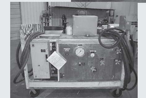
A&P Hydraulics Mdl 03-510-05 Skydrol Hydraulic Test Cart, Max Pressure 5,500 PSI, Max Flow 25 GPM
