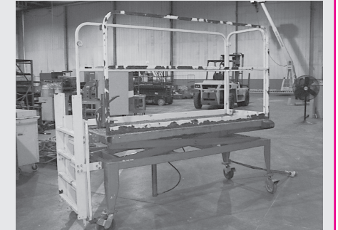
(2) Tronair B4 Maintenance Stands 04-6029-5111 & -5112, 41" Platform Lowered Height, 7' Platform Raised Height, 9' Long, 500 Lb Capacity (2) Bombardier Wheel & Brake Dollies
