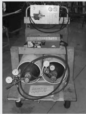
2-Bottle Tow Behind Nitrogen Cart w/ Tronair Mdl 99-9003-1100 High Pressure Nitrogen Gas Booster
