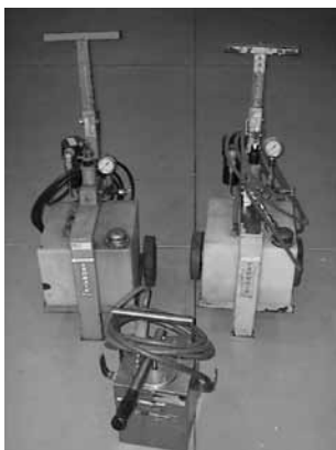
(2) Tronair Mdl's 06-4035-0500, 06-4035-3600 Hydraulic Service Units, 8-Gal Capacity Tronair Mdl 06-5022-6500 Hydraulic Service Unit, 2-Gal Cap
