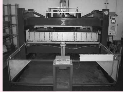
Hall Dielectric Machinery Co. Mdl. FS-40 Radio Frequency Heat Sealing Machine. S/N 1643, 40 kw RF Power Output, Freq. 27.12 Mhz, Bed Plate 96" x 56", Heated Platen 90" x 50", Throat Size 32 1/2"
