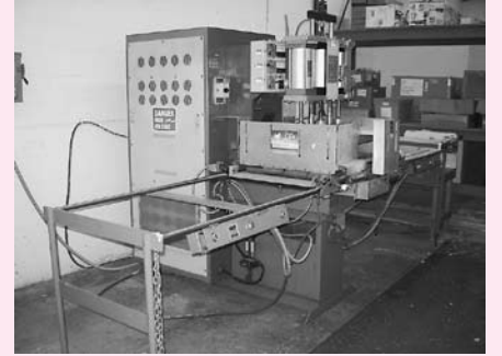
(2) Hall Dielectric Machinery Co. Mdl. FS-15A Radio Frequency Heat Sealing Machine, 15 kw RF Power Output, Freq. 27.12 Mhz, Bed Plate 33" x 27", Heated Platen 24" x 20", Throat Size 16 1/2", 8" Stroke, 2827 Lbs Down Pressure at 100 PSI, Manual Side to Side Slide Tray Shuttle
