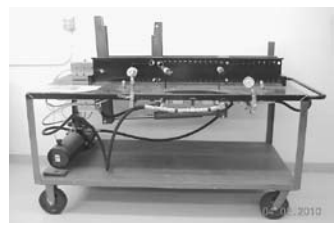
Electrical Mechanical Actuator Test Stand 15 HP Dual Head Low-1,100-5,500 RPM, Vari Drive High 2,400-12,000 RPM Blue Wave Ultrasonic Cleaning Bench, 18' L x 12' W x 10' D Tank
