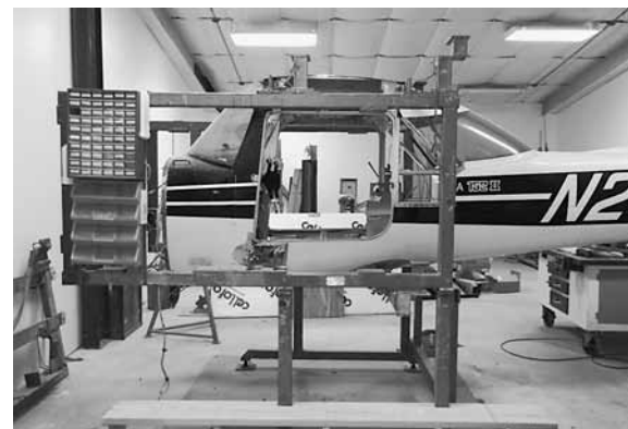
Cessna Factory Fuselage Jig, 100 & 200 Series Cessna Factory Wing Jig, 100 & 200 Series
