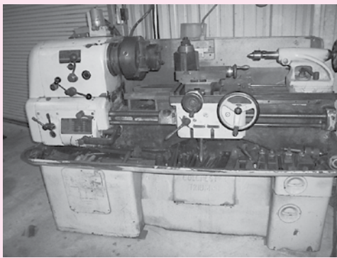
Colchester Triumph Gap Bed Lathe, 12" Swing over Bed, 24" Gap Sing, 27" Between Centers, 45" Bed, 2" Hollow Spindle w/Variou Chucks, Tool Holders & Cutters
