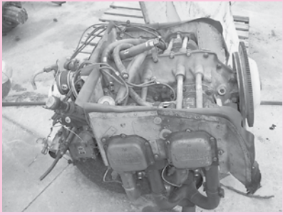
Lycoming O-360-A4K Engine Core w/All Accessories
