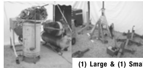
Devilhiss 15 HP Dual Style Horizontal Air Compressor Ingersoll Rand 5 HP Dual Stage Vertical Air Compressor
