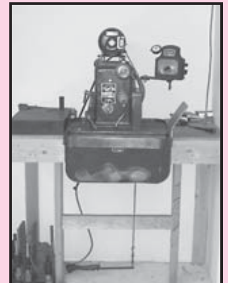
Sunnen Mdl. #LBA650 Horizontal Hone w/Mandrels and Sunnen Mdl. #AG-300 Precision Gauge
