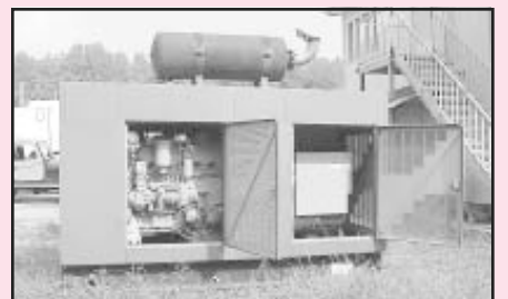
Caterpillar Generator Set, Has Cat 3406 Diesel Engine, Generator Rating 375 K.V.A., 300 K.W., 60 Hertz with Large Fuel Tank Platform
